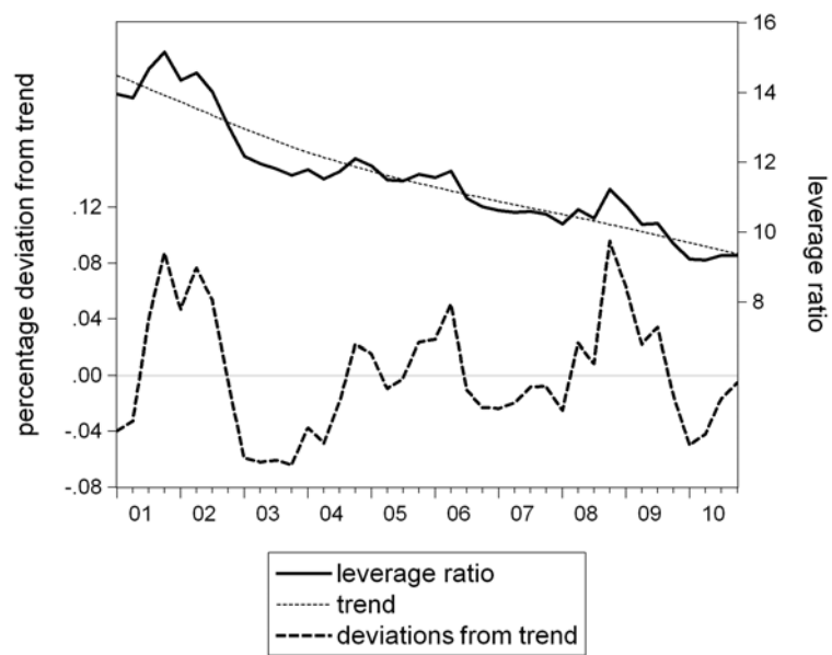
Figure 3: Mexican leverage ratio, 2001q1 - 2010q4
