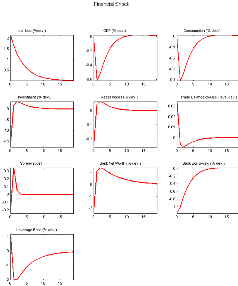
Figure 5: IRFs to a financial shock
