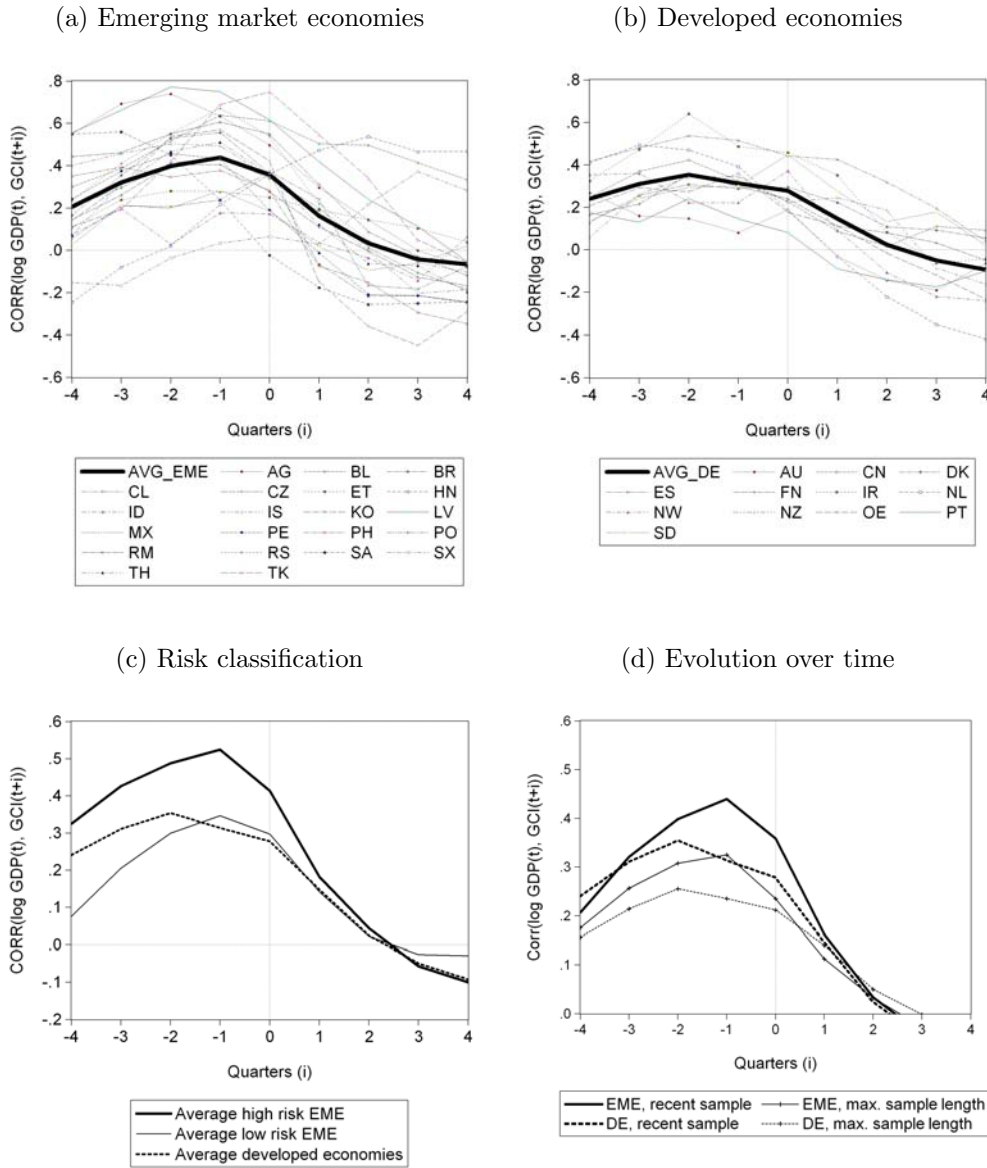
Figure 2: Lead-lag structure of cross-correlations.
