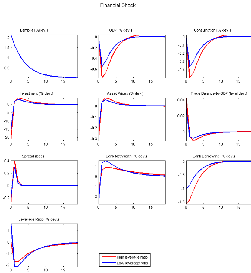
Figure 7: Sensitivity 2: IRFs to a financial shock with different leverage ratios.
