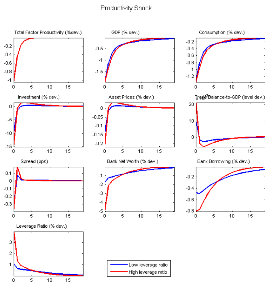
Figure 6: Sensitivity 1: IRFs to a productivity shock with different leverage ratios.
