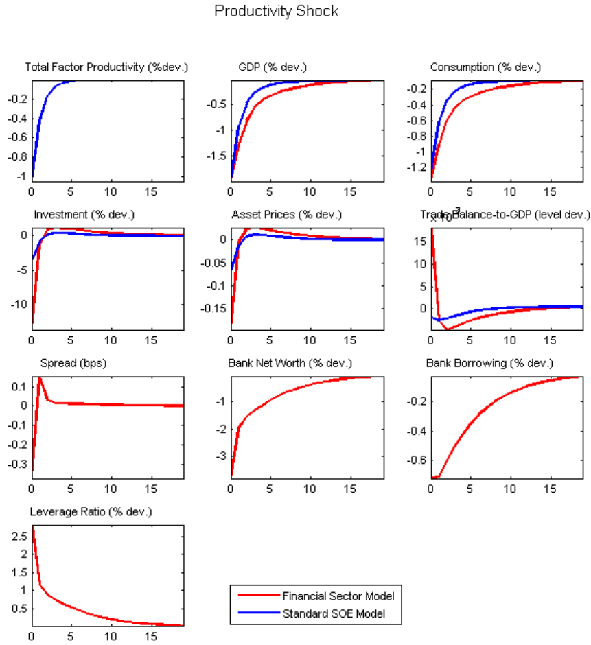
Figure 4: IRFs to a productivity shock
