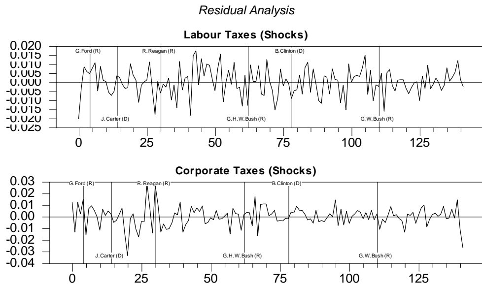
Figure 9: Residual Analysis (7-SVAR: Labour, Corporate and Indirect Taxes)
