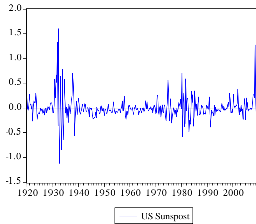
Figure 5: Sunspots
