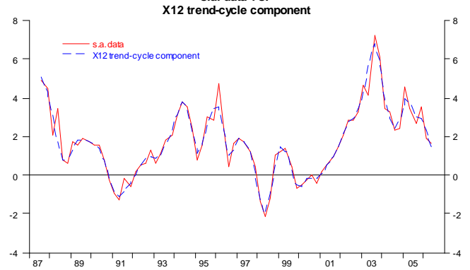
Correlation with QPC GDP
