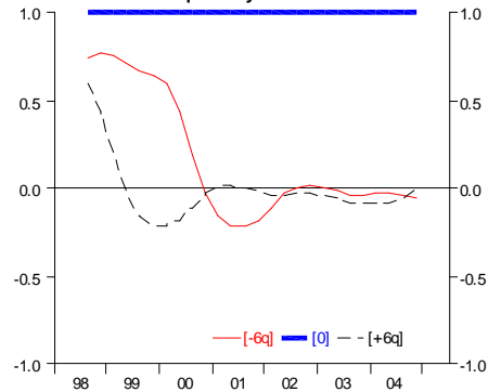
Rolling (40q) correlation with qtrly non-tradables inflation
