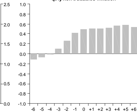
Correlation with 90 day rate gap
