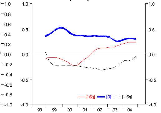
Rolling (40q) correlation with qtrly non-tradables inflation
