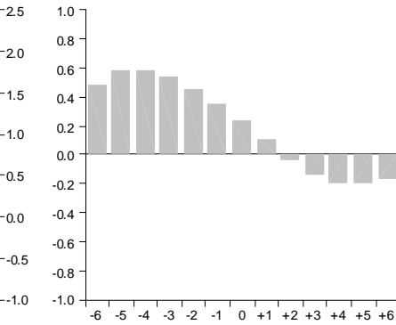
Correlation with quarterly CPI inflation
