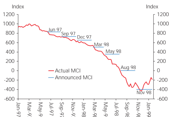
Figure 1: Actual and announced MCI developments since 1997
