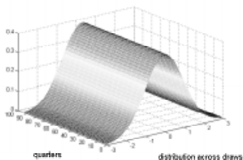
Figure 2: Hypothetical distributions across draws
